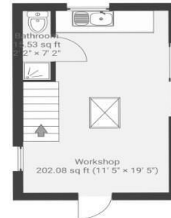
STUDIO GROUND FLOOR
